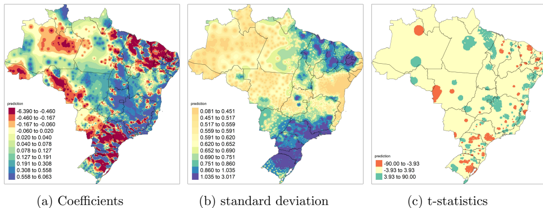
Figure 7: \beta_1 estimates GWR, IDHM - Instrumentalized IQIM.
