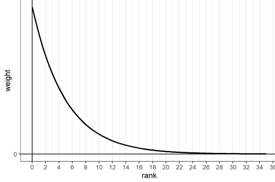
Figure 3: exponential function weights
