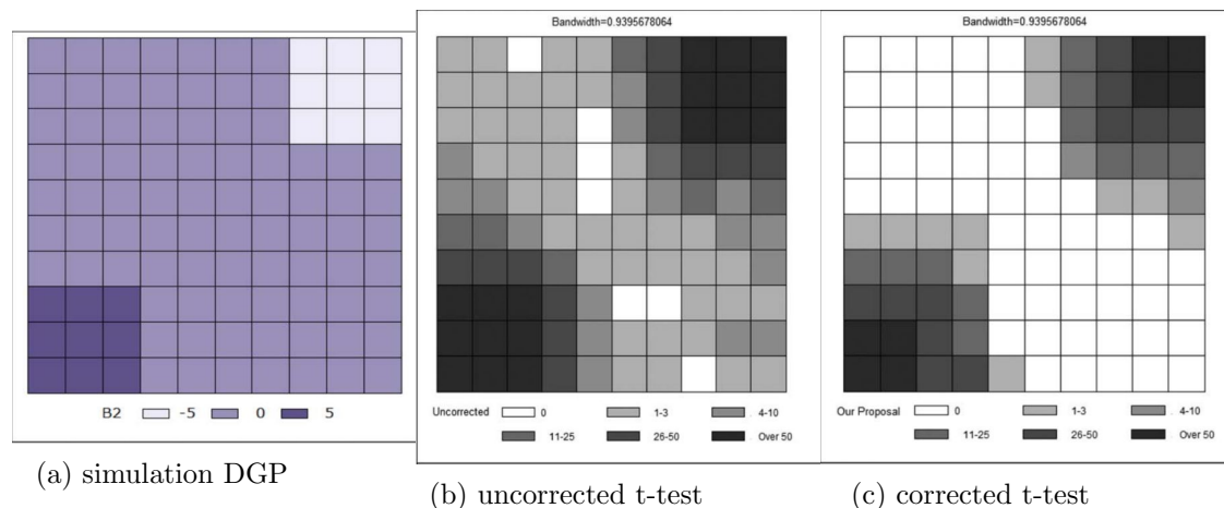
Figure 4: Simulation comparison of corrected and uncorrected t-test
