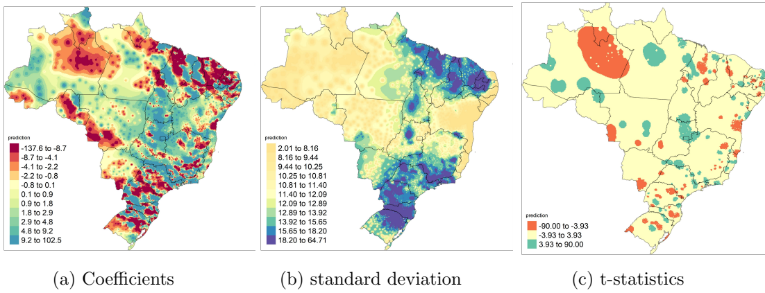
Figure 9: \beta_1 estimates GWR, Education - Instrumentalized IQIM.
