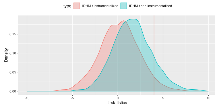
Figure 19: Density instrumentalized and non-instrumentalized t-statistics
