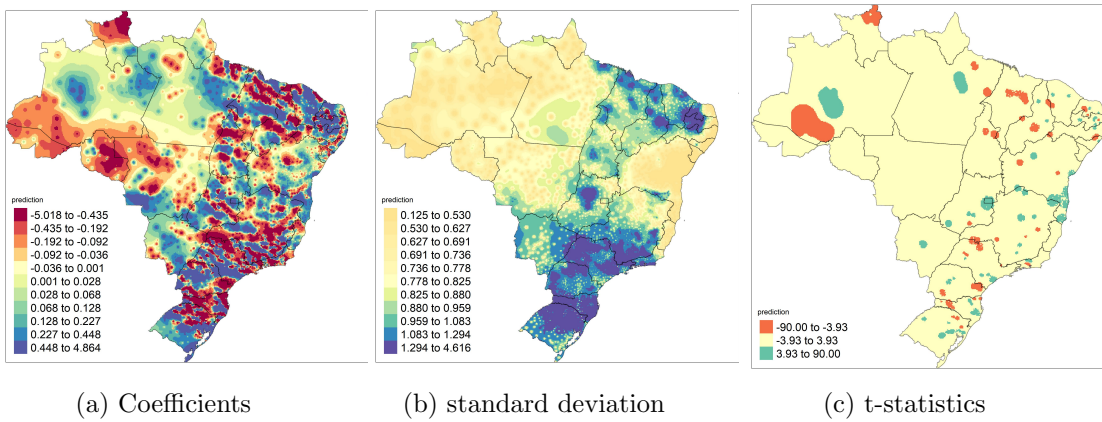
Figure 10: \beta_1 estimates GWR, GINI - Instrumentalized IQIM.
