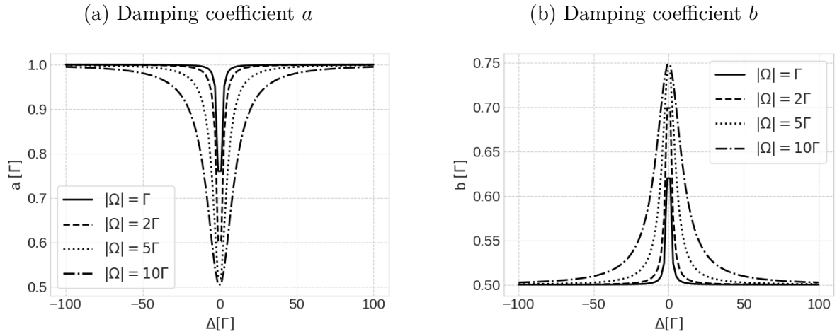
Figure 7 – Damping coefficients a and b from equation (2.71) as a function of the detuning \Delta for different Rabi frequencies \Omega .
