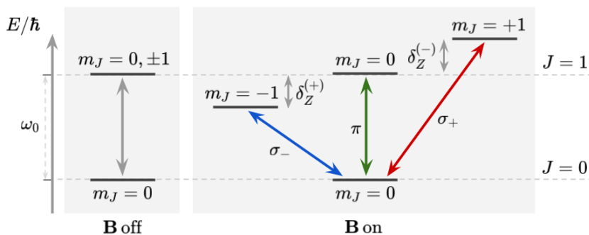
Figure 14 – Zeeman splitting of the transition J = 0 \rightarrow J = 1 in 1D-MOTs. When \mathbf{B} = 0 ( B off ), the atomic transition J = 0 \rightarrow J = 1 is described by a degenerate two-level system . However, when \mathbf{B} \neq 0 ( B on ), the same atomic transition is represented by a four-level system in which the excited states are energetically separated by the Zeeman shift \delta_Z^{(\pm)} . The energy scale was not plotted precisely to enhance the visibility.
