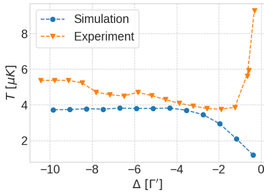
(a) Temperature vs. laser detuning.
