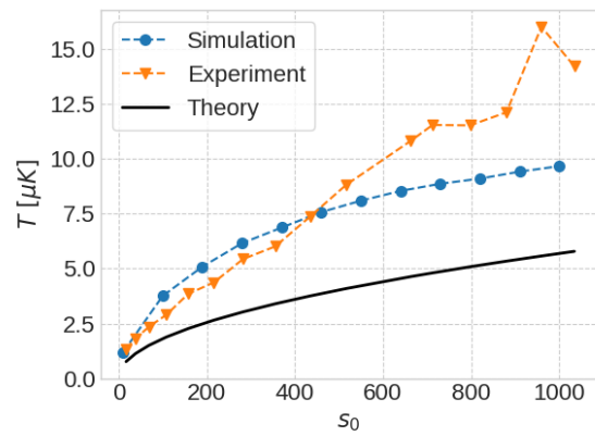
(b) Temperature vs saturation parameter.
