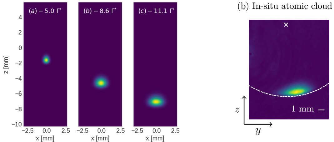
(a) Simulated atomic cloud
