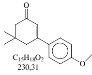
3-(4-metoxifenil)-5,5-dimetilciclohex-2-enona
