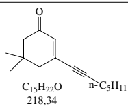
3-(hept-1-ynyl)-5,5-dimethylcyclohex-2-enona
