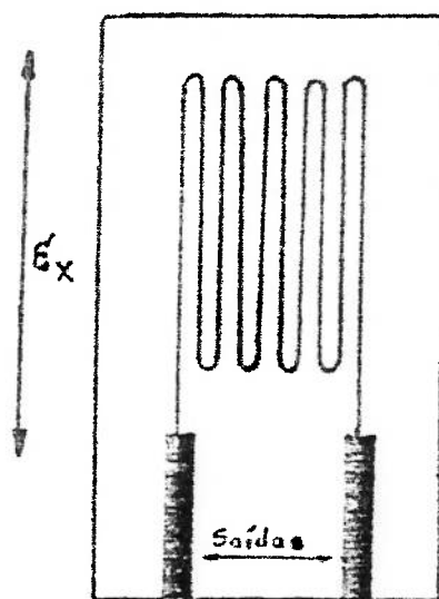
Fig.B.1 Strain gage
