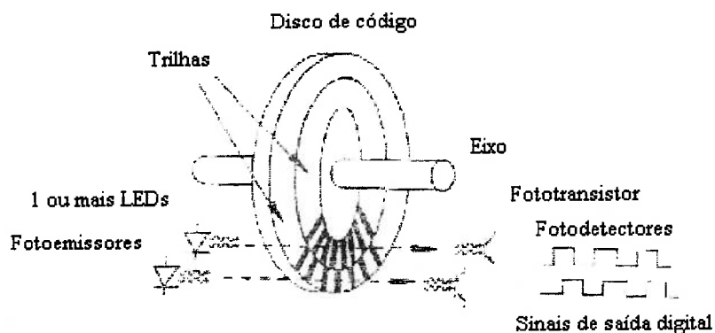
Fig.A.1 Encoder
