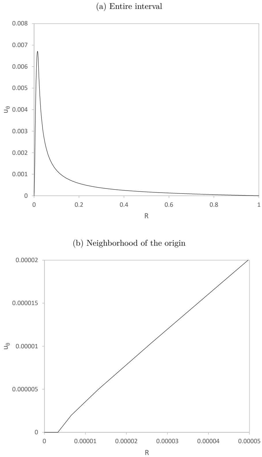
Figure 41 – Tangential displacement u_\theta of the artifact of the numerical procedure.
