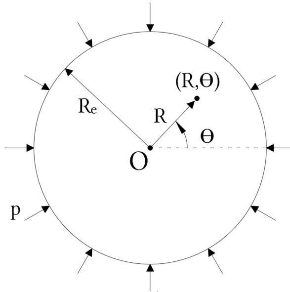
Figure 4 – Anisotropic disk compressed by a uniform pressure along its external boundary.
