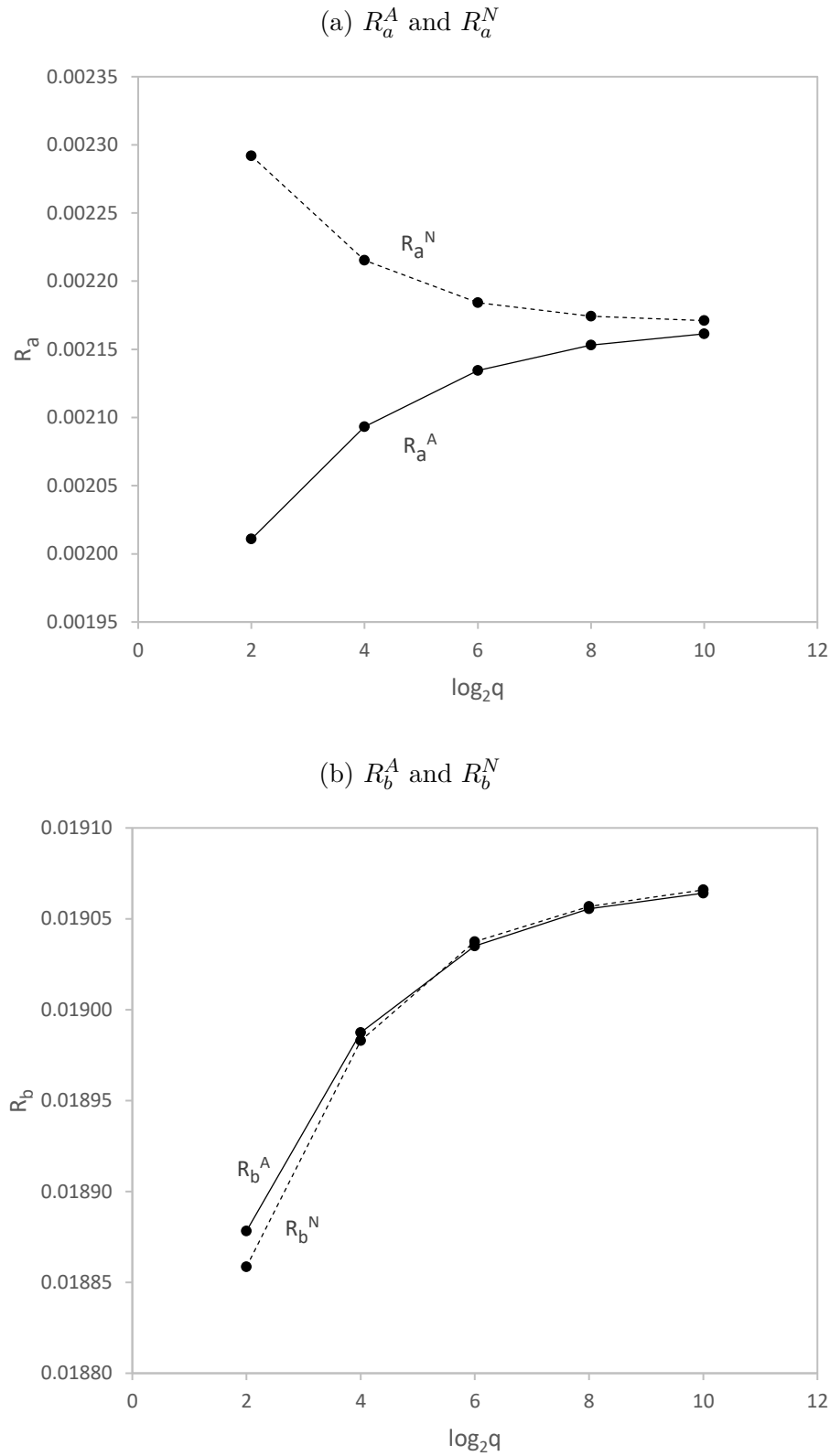
Figure 44 – Approximations of the radii R_a and R_b versus the base 2 logarithm of the mesh parameter q = 4, 16, 64, 256, 1024 .
