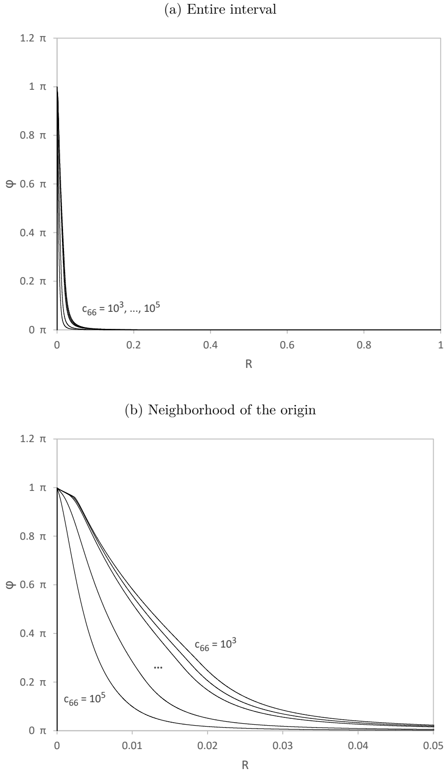
Figure 29 – Angle of rotation \varphi obtained from the rotationally symmetric solution for increasing values of c_{66} and for \delta = 10^8 .
