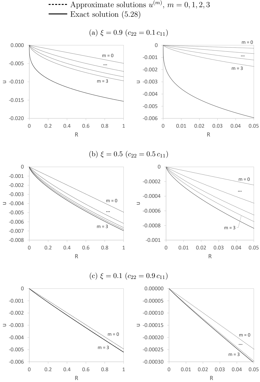
Figure 10 – Radial displacement u versus radius R for unconstrained disk problem considering the cases \xi = 0.9, 0.5, 0.1 .
