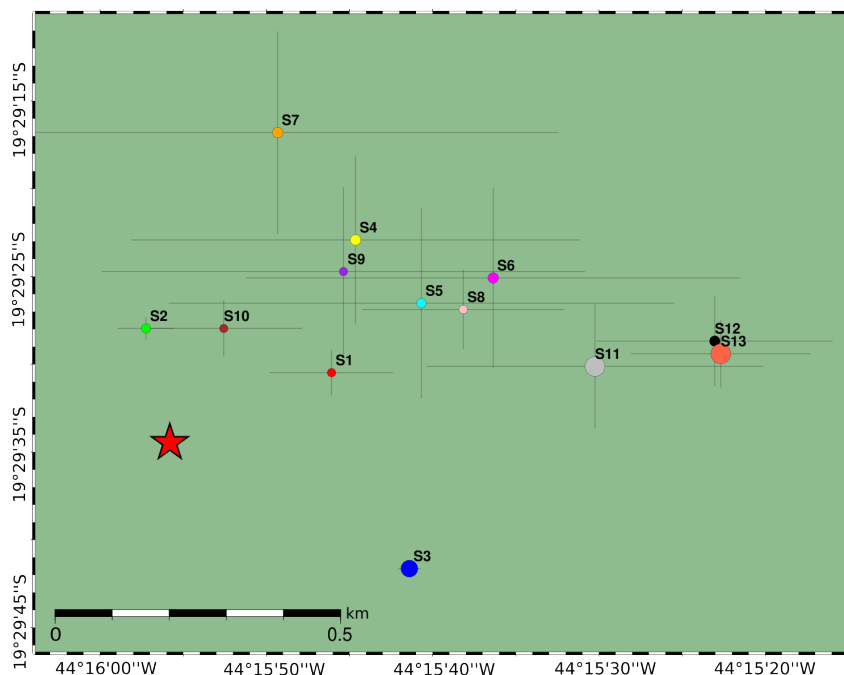
Figure 5.9: Location of Sete Lagoas events. Red star is the reference (Master) event and circles the located target events using only P- and S-waves. The errors are larger due to the limited number of stations. Events S3, S6, and S12 have different locations in comparison to Figs. 8, 9, and 10.
