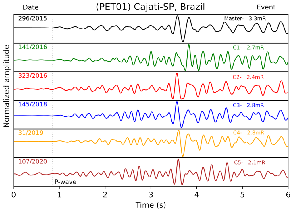
Figure 6.4: Waveforms of the mainshock and five aftershocks near Cajati showing a noticeable similarity. ON.PET01 station (98km), vertical component velocity records, band-pass filtered (2-8Hz). The event times (day of year/year) are displayed in the left corner, while the event number and magnitude are shown in the right corner. The dashed line indicates the P-wave arrivals.
