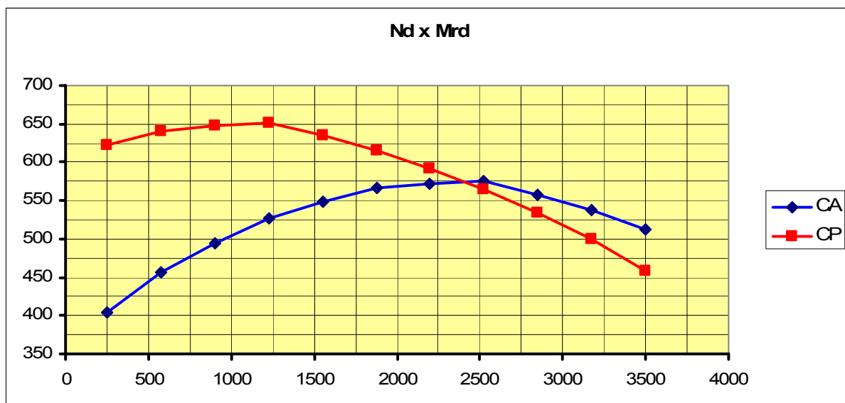
Figura 6.21 – Curva N_d \times M_{rd} do pilar
